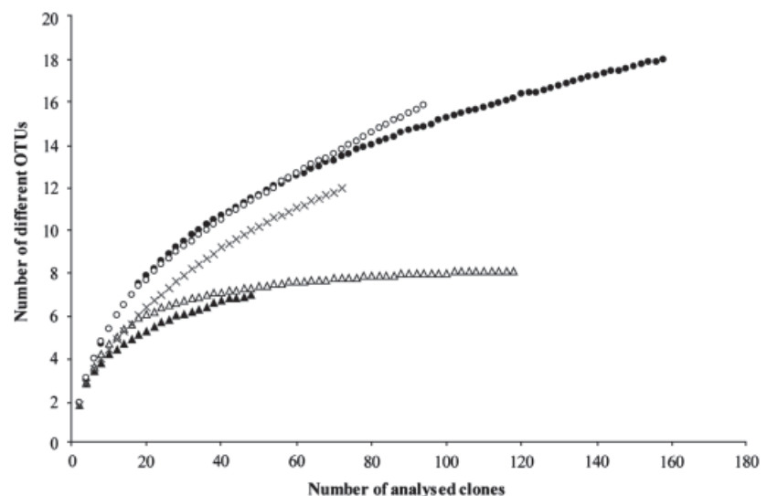
Fig. 1. Rarefaction curves for results obtained from the community analysis of the Blue Lagoon using culture-independent techniques. Symbols: \Delta , summer 2003; \blacktriangle , summer 2005; \bullet , autumn 2003; \circ , autumn 2005; \times , winter 2006.
